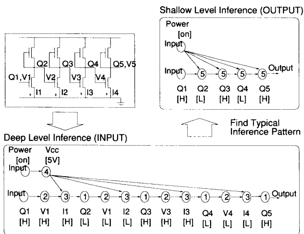
Fig. 3 CLIP: Concept Learning from Inference Pattern.
